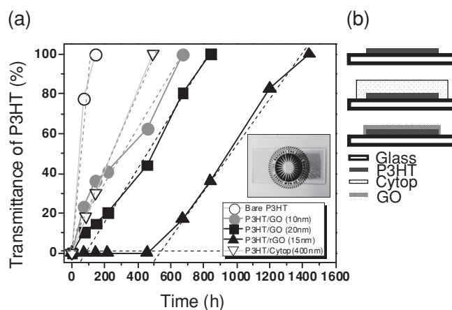
Figure 1. Gas barrier property of GO/rGO films measured by P3HT transmittance test. a) P3HT films on glass substrates were encapsulated with GO and rGO, and compared with controls. The inset shows a photograph of the GO films used for encapsulation on glass (left), and GO encapsulated P3HT films demonstrating high optical transparency of GO films used in this study (right). Dashed line fits used to extract the slope values for calculation of diffusivity in the steady-state flux regime are also shown. b) Schematic of sample structures used for the P3HT transmittance tests.
